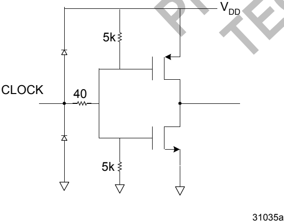
Figure 6. Equivalent Encode Input Circuit
