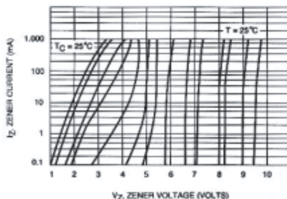
Figure 7. Zener Voltage versus Zener Current V_Z = 6.8 thru 10 Volts
