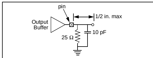
Figure 1-6. PCI T_{val(max)} Rising Edge
