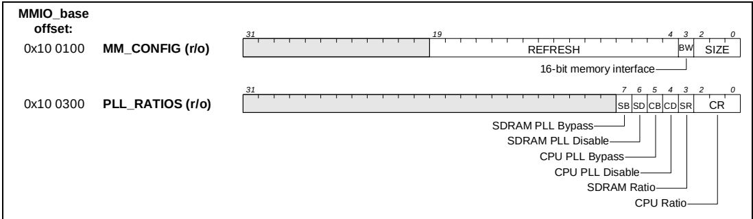
Figure 12-2. Memory interface configuration registers.
