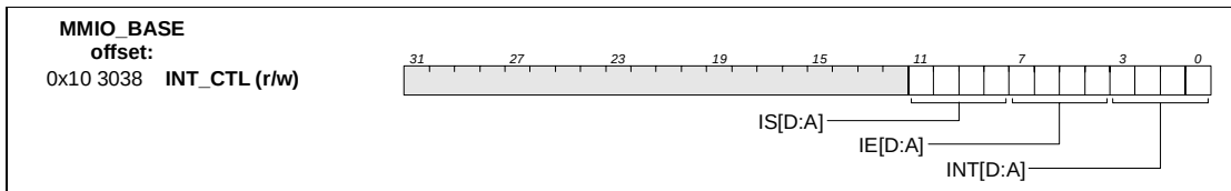
Figure 3-9. Host interrupt control register
