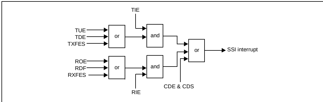
Figure 17-8. Interrupt generation logic.
