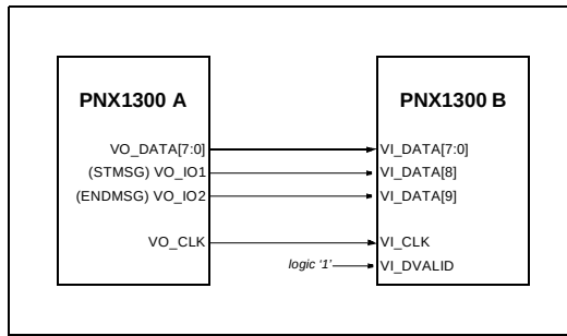
Figure 7-3. EVO unit connected to the VI unit of a second PNX1300.
