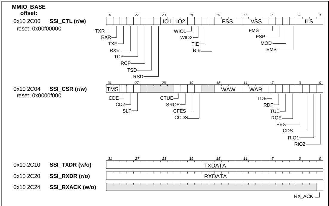
Figure 17-10. SSI MMIO registers.
