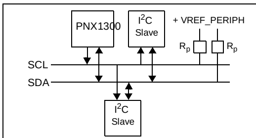
Figure 16-1. Typical I 2 C system implementation
