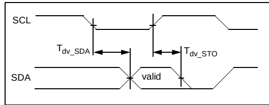
Figure 1-15. I²C I/O Timing
