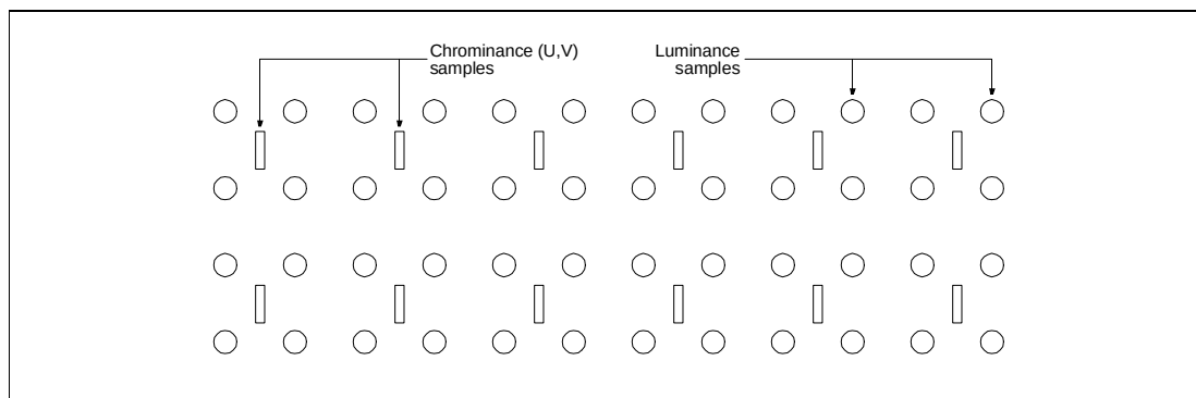
Figure 7-21. YUV 4:2:0 format.
