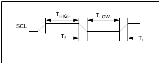
Figure 1-11. I²C I/O Timing
