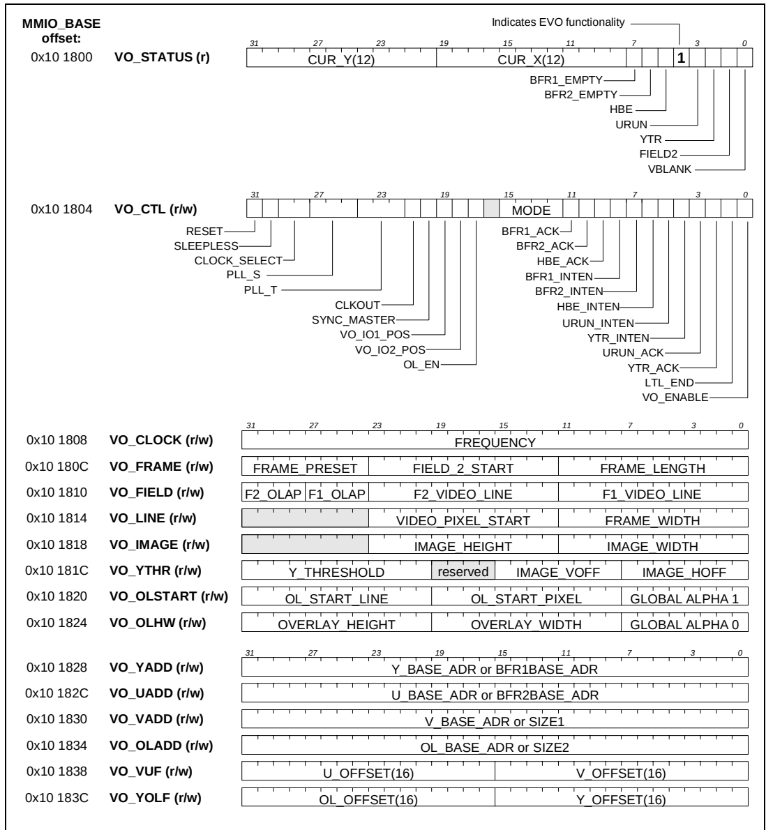
Figure 7-29. EVO MMIO registers.
