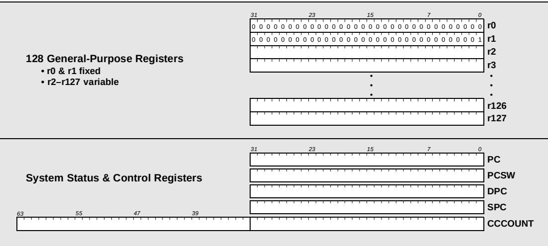
Figure 3-1. PNX1300 registers.
