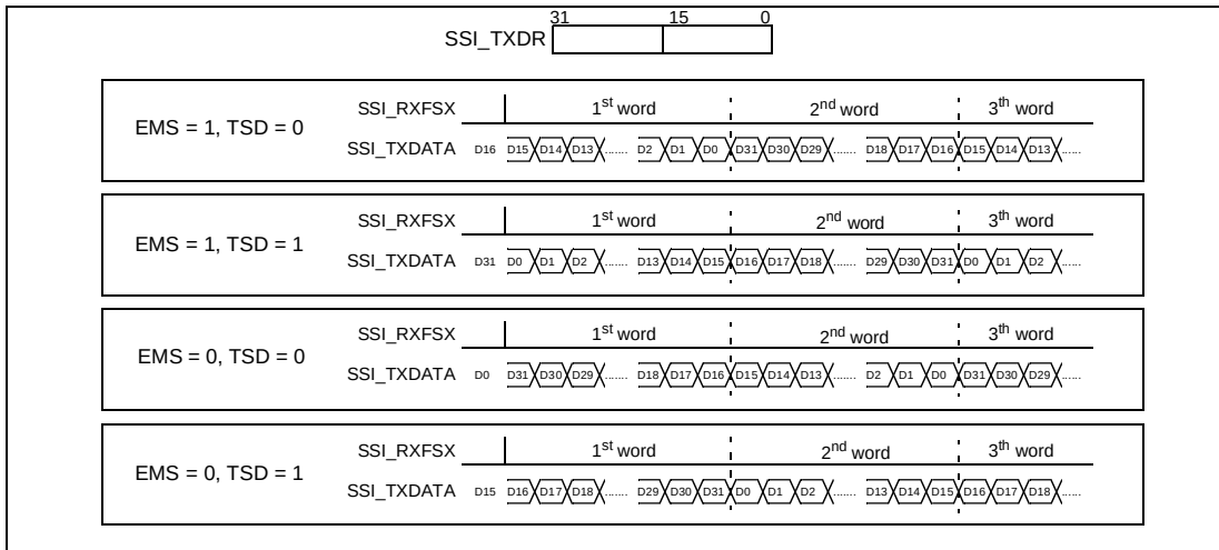
Figure 17-9. 16-bit endian and shift direction operation.
