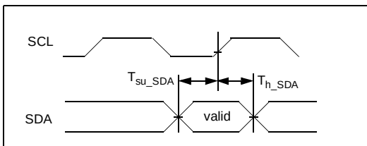
Figure 1-14. I²C I/O Timing
