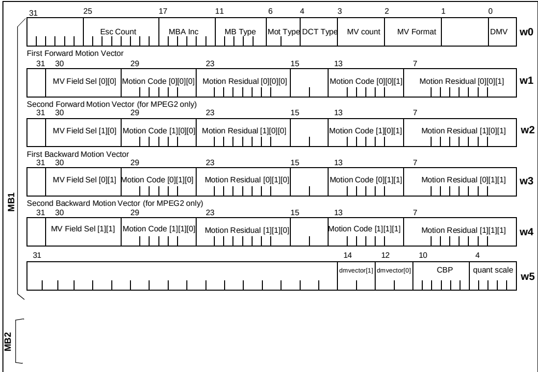
Figure 15-2. MPEG-2 macroblock header output format
