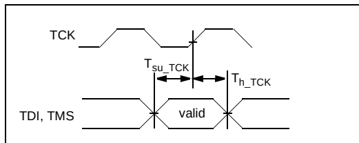
Figure 1-9. JTAG Input Timing
