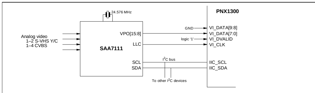
Figure 6-3. VI unit connected to a video decoder.
