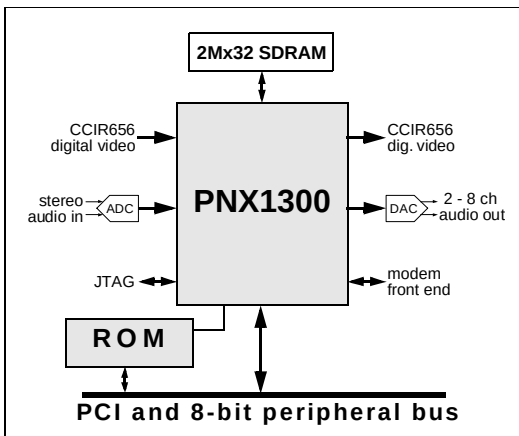
Figure 2-2. PNX1300 system connections. A minimal PNX1300 requires few supporting components.
