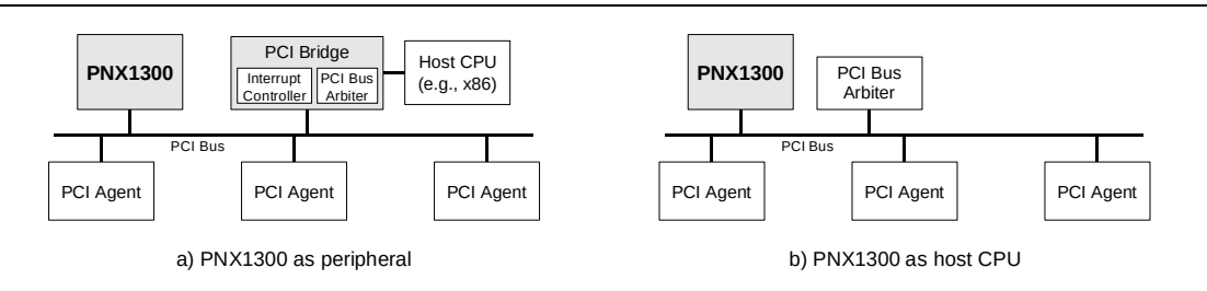
Figure 11-1. Two typical system implementations: (a) shows PNX1300 as a PCI peripheral in a desktop PC, (b) shows an embedded system with PNX1300 as the host CPU.
