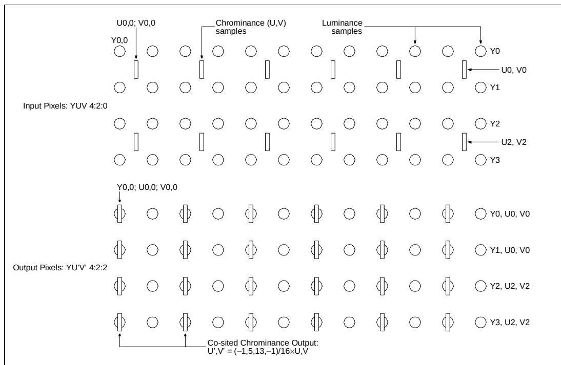
Figure 7-25. YUV 4:2:0 to YUV 4:2:2 co-sited conversion.
