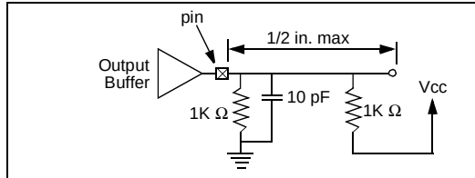
Figure 1-8. PCI T_{val(min)} and Slew Rate
