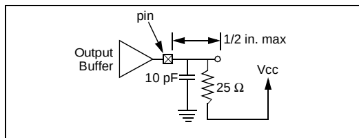
Figure 1-7. PCI T_{val(max)} Falling Edge
