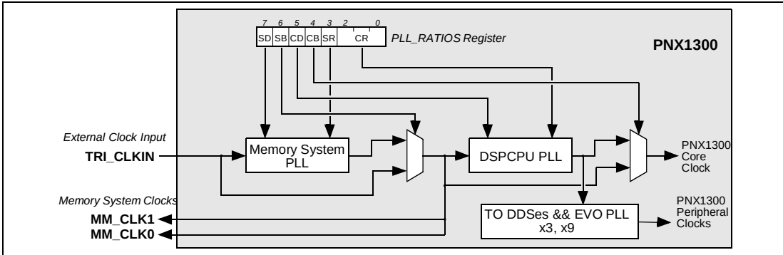
Figure 12-3. PNX1300 memory and core PLL connections.
