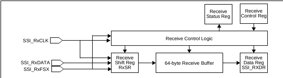
Figure 17-5. The SSI receive block diagram
