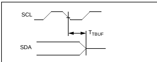
Figure 1-12. I²C I/O Timing
