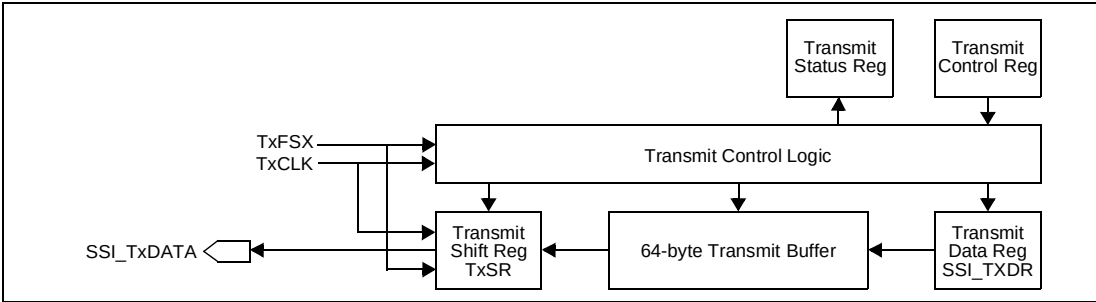
Figure 17-4. The Sync Serial Interface Transmit Block Diagram
