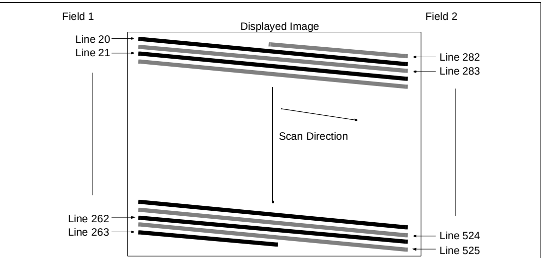
Figure 7-9. Interlaced display: 525-line, 60-Hz image.
