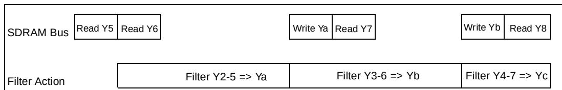
Figure 14-15. SDRAM and vertical filter block timing
