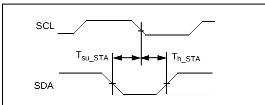
Figure 1-13. I²C I/O Timing
