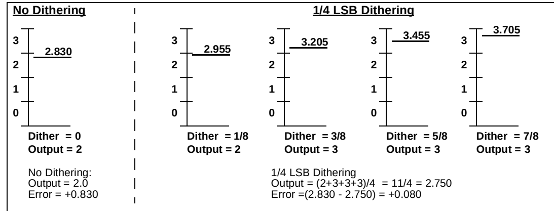
Figure 14-10. Dithering
