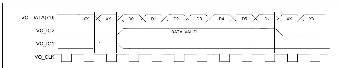
Figure 7-17. Data-streaming valid data signals.
