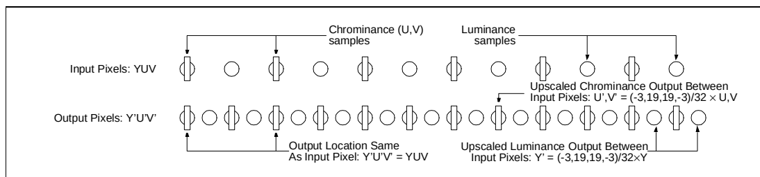
Figure 7-26. 2x upscaling of Y pixels.
