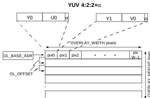
Figure 7-23. YUV 4:2:2+alpha overlay format.
