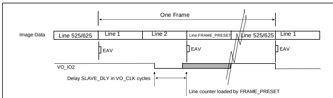
Figure 7-16. Genlock mode.
