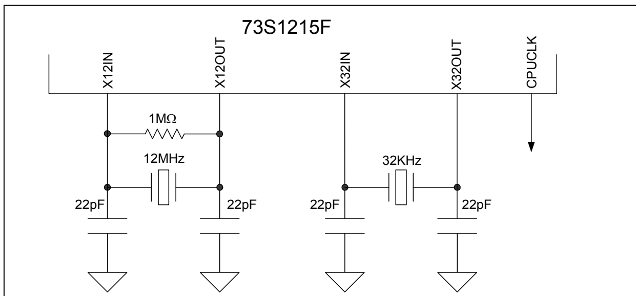
Figure 4: Oscillator Circuit
