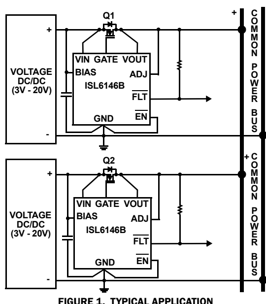
FIGURE 1. TYPICAL APPLICATION
