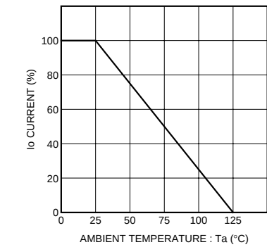
Fig. 4 Derating curve (mounting on glass epoxy PCBs)
