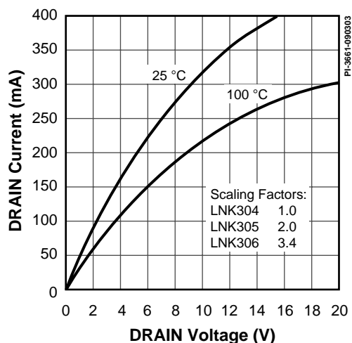
Figure 15. Output Characteristics.
