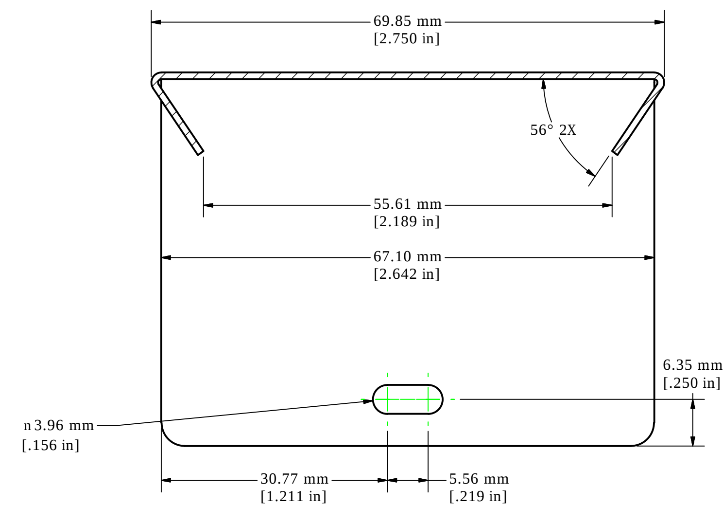
BOTTOM VIEW OF ASSEMBLY
