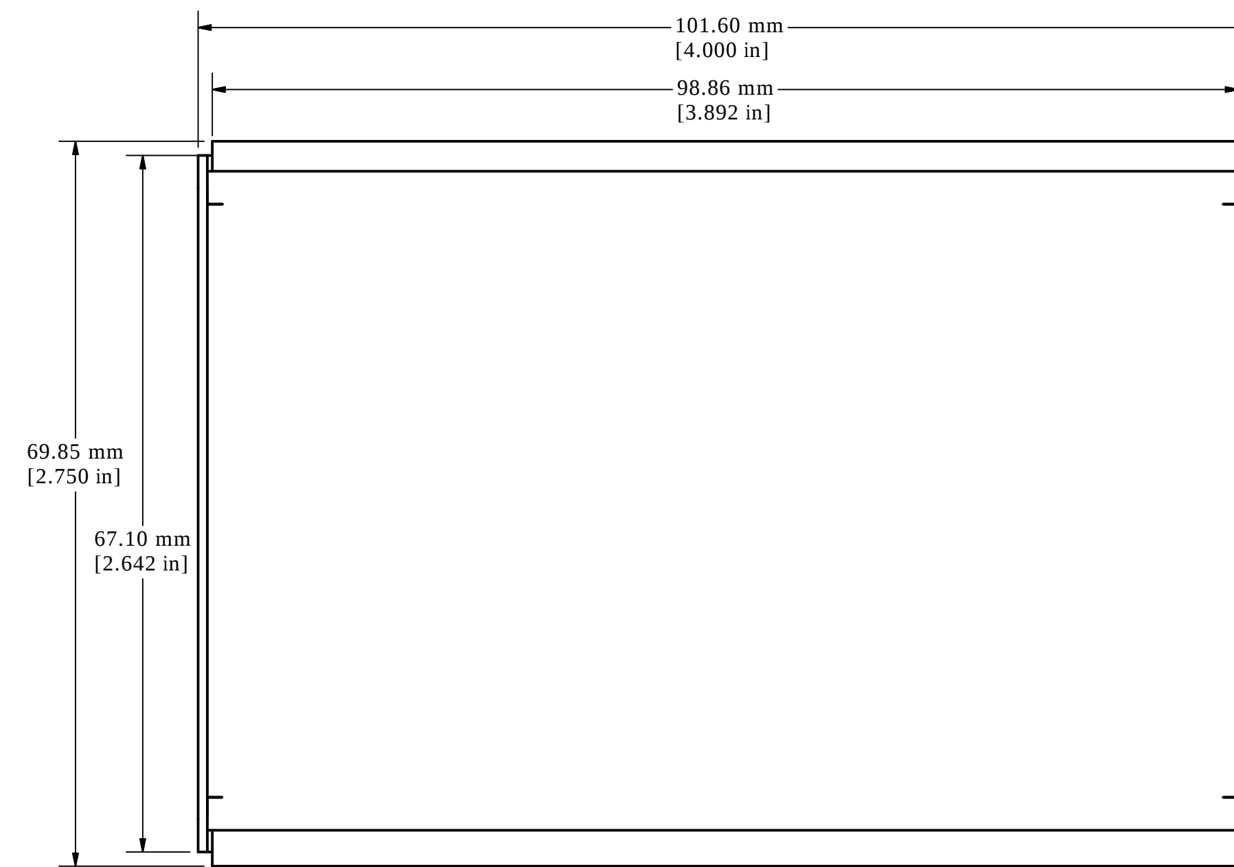
BOTTOM VIEW OF ASSEMBLY
