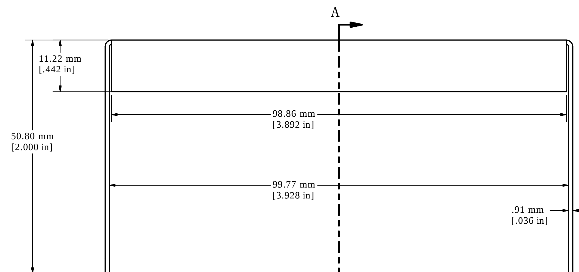
TOP VIEW OF ASSEMBLY
