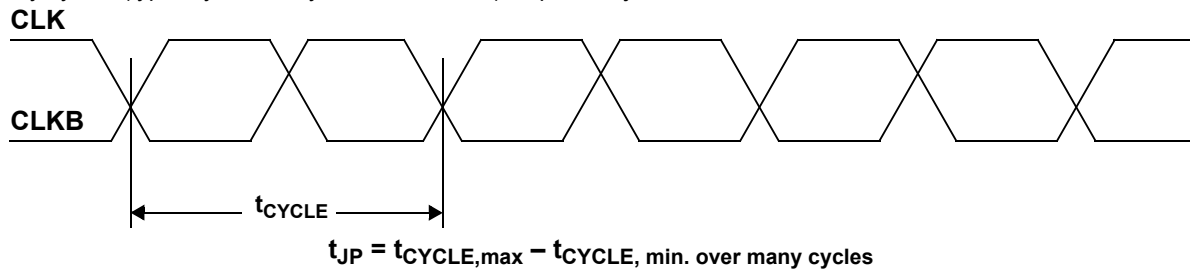
Figure 6. Period Jitter
