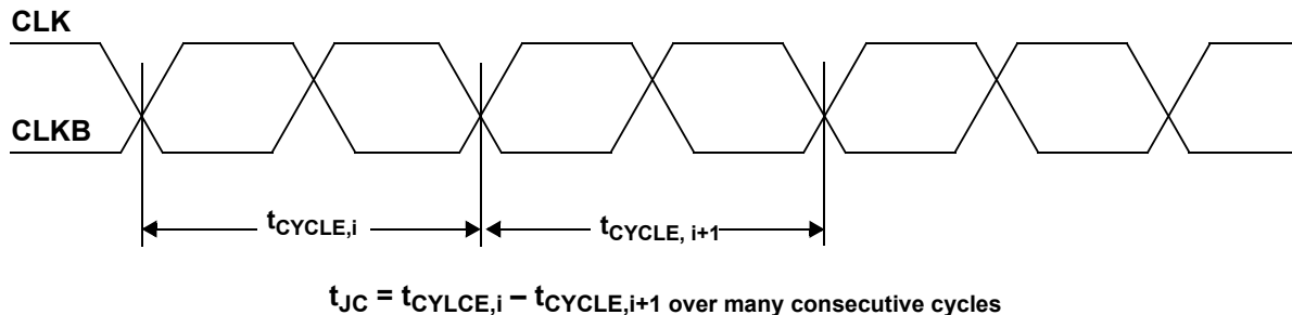
Figure 7. Cycle-to-cycle Jitter
