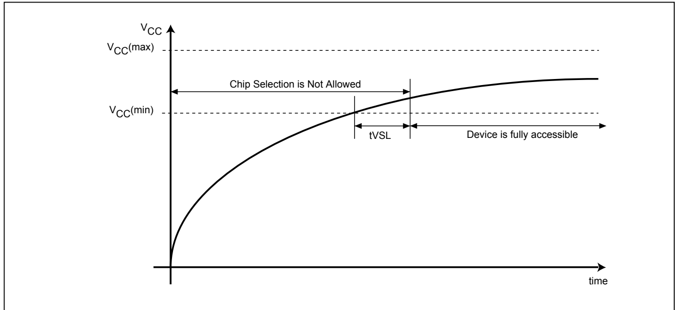
Figure 52. Power-Up Timing
