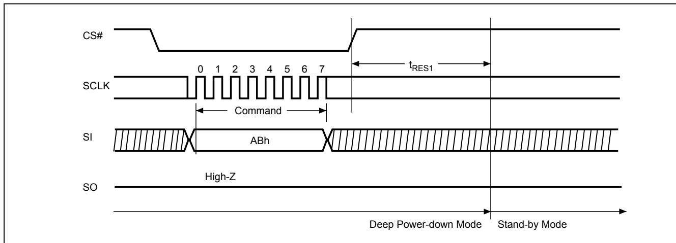
Figure 29. Release from Deep Power-down (RDP) Sequence (Command AB)
