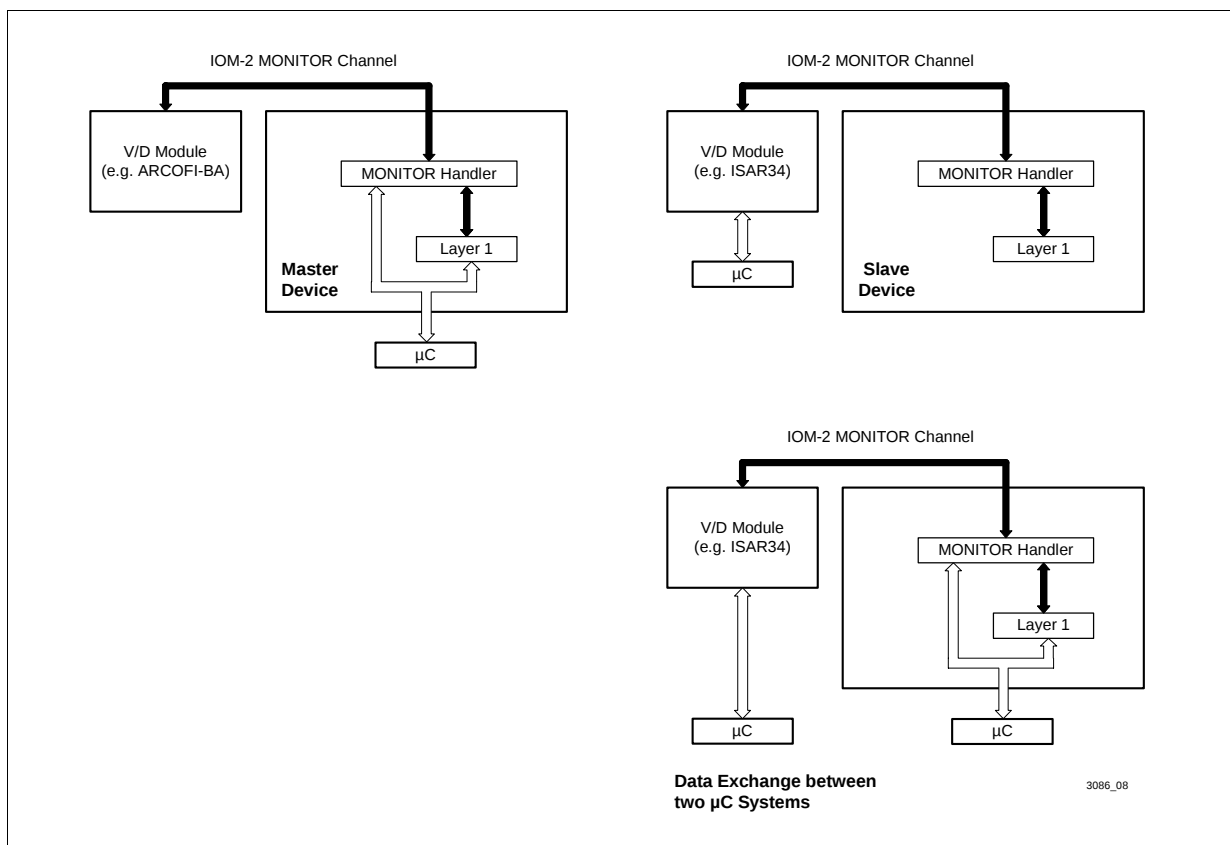
Figure 52 Examples of MONITOR Channel Applications in IOM-2 TE Mode
