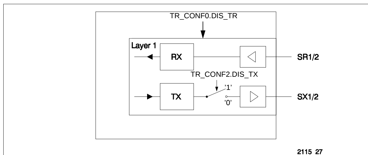
Figure 26 Disabling of S/T Transmitter
