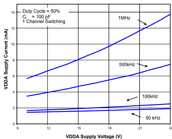
Figure 3.25. Supply Current vs. Supply Voltage
