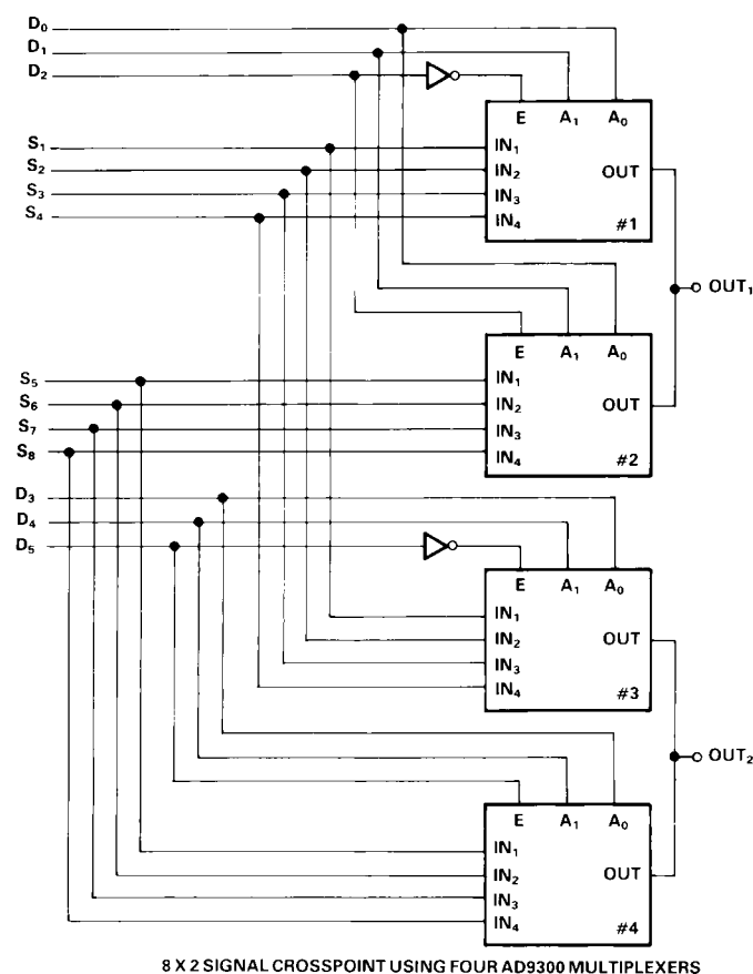
Figure 11. 8 \times 2 Signal Crosspoint Using Four AD9300 Multiplexers
