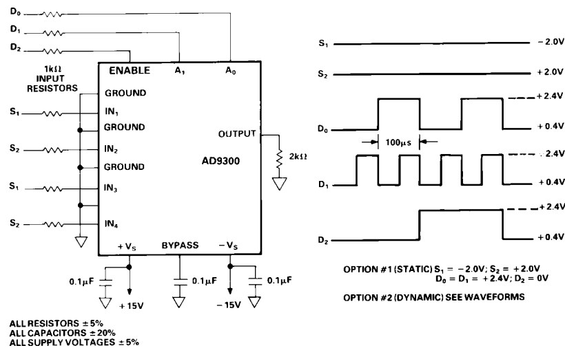
AD9300 BURN-IN DIAGRAM
