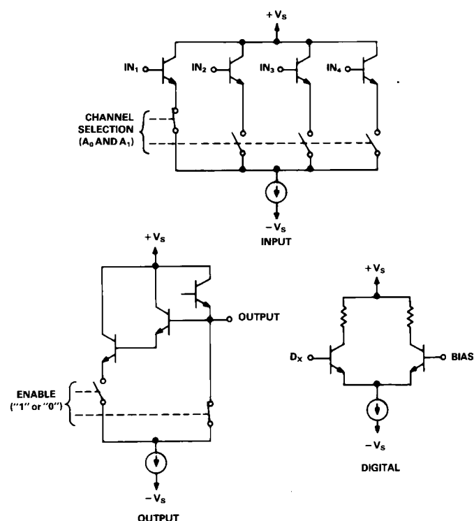
Figure 1. Input and Output Equivalent Circuits
