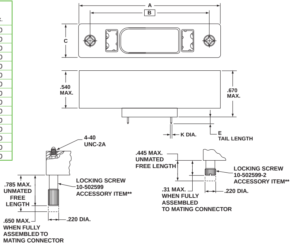
Input/Output Connector
