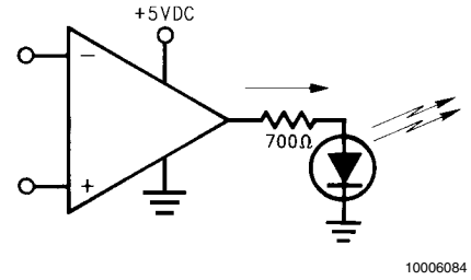
FIGURE 23. LED Driver
