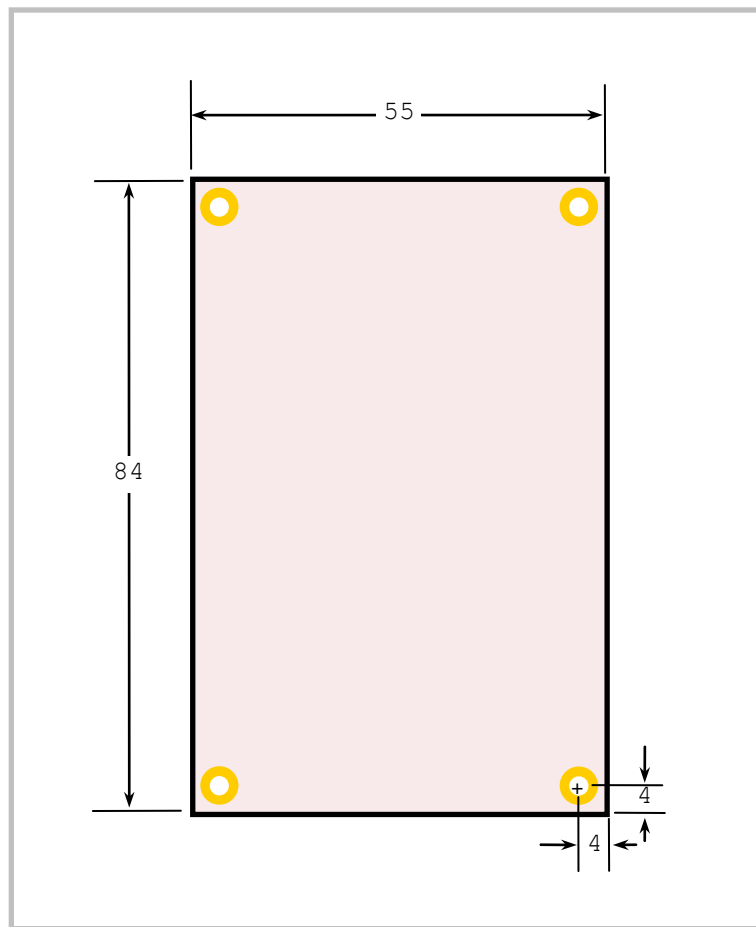
Figure 4. Falcon Dimensions and Mounting Holes (Not to scale. All dimensions in millimeters.)
