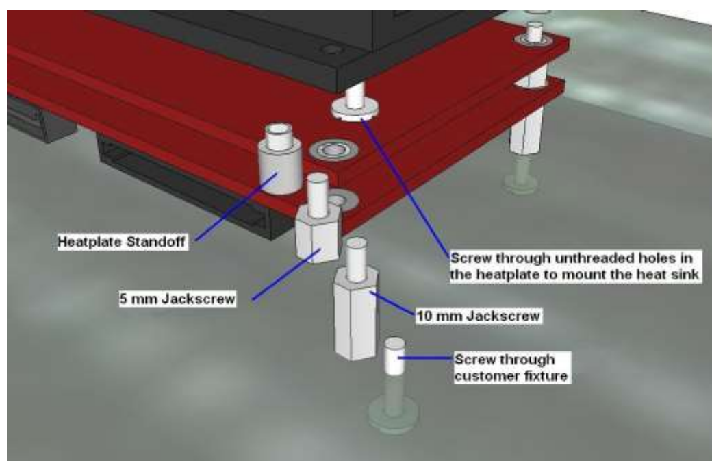
Figure 14. Bolt-through Heatsink
