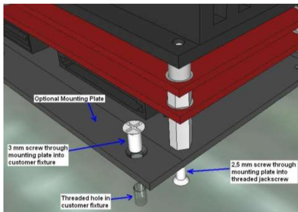
Figure 15. Mounting Plate Option 1
