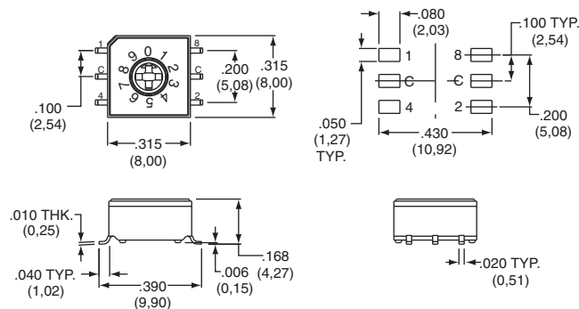
CD10RM0SB
