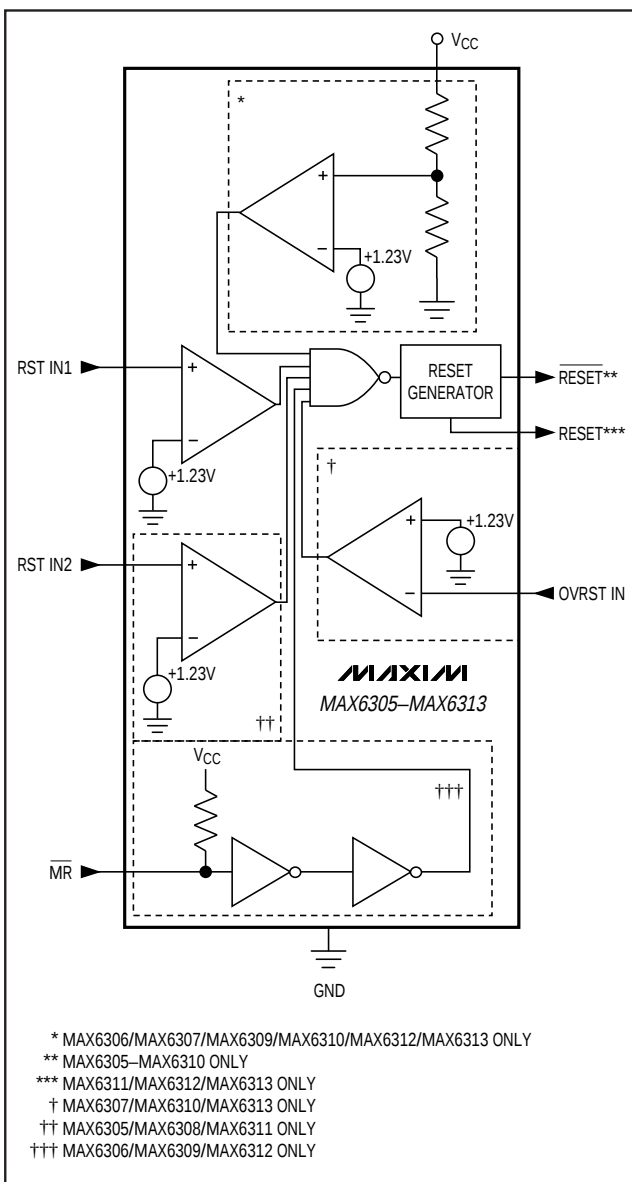
Figure 1. Functional Diagram
