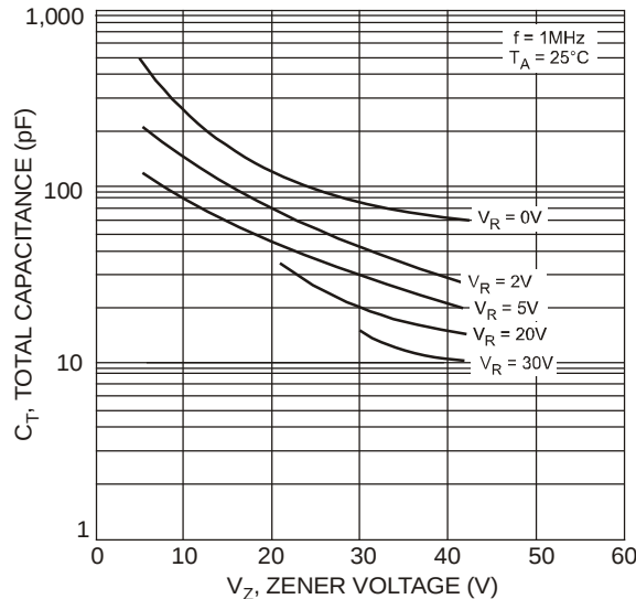
Fig. 3 Typical Total Capacitance vs. Zener Voltage
