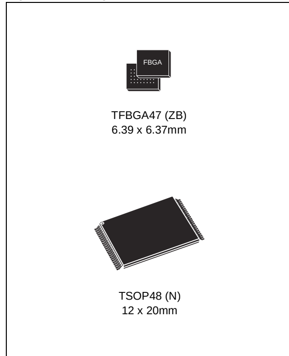
Figure 1. Packages
