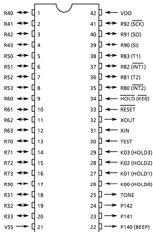
(1) SDIP42-P-600-1.78
