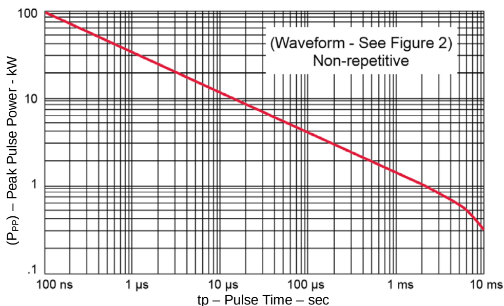
FIGURE 1 Peak Pulse Power vs. Pulse Time
