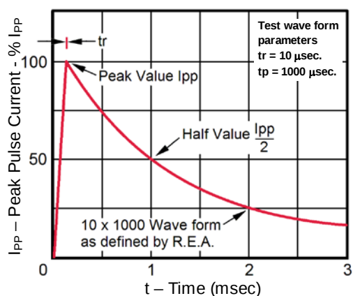
FIGURE 2 Pulse Waveform
