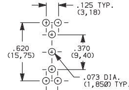
8161SH9_BE2 SPDT
