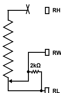
FIGURE 18. DCP CONNECTION IN SHUTDOWN MODE
