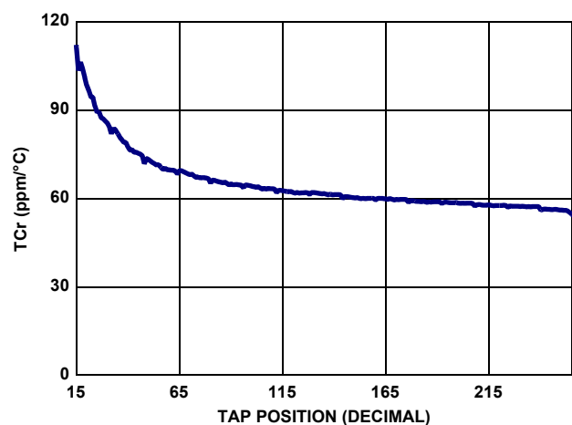
FIGURE 11. 100k TCr vs TAP POSITION
