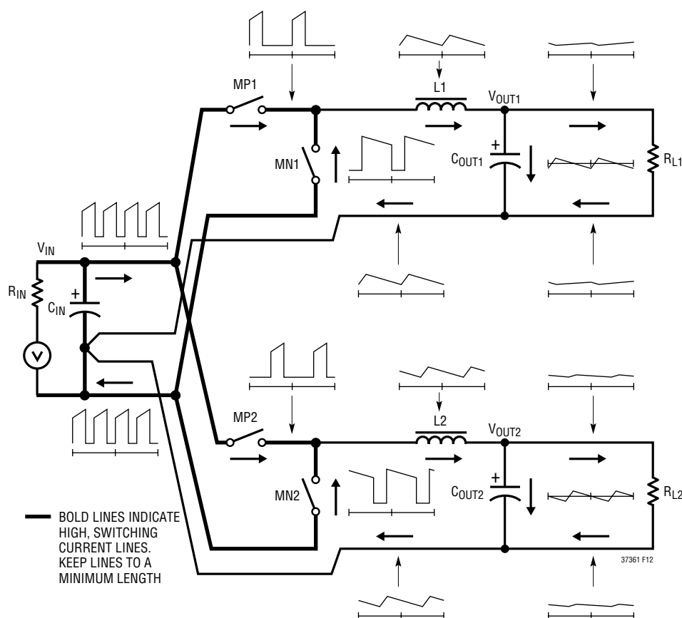
Figure 12. Branch Current Waveforms
