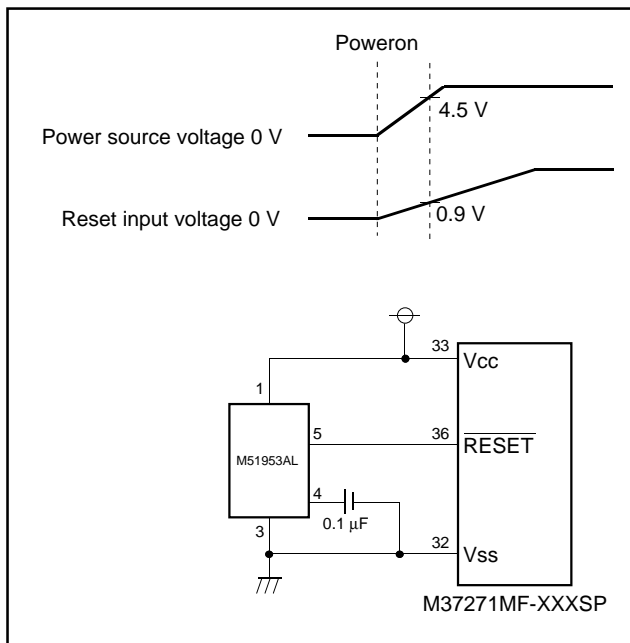
Fig. 89. Example of reset circuit
