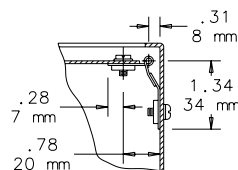
DETAIL X 87799584
