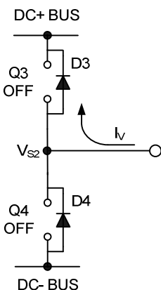
Figure 23: D3 conducting
