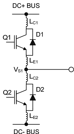
Figure 25: Parasitic Elements
