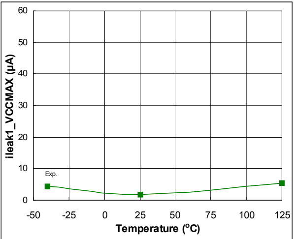
Fig. 57. Offset Supply Leakage Current vs. Temperature
