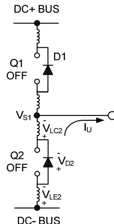
Figure 27: V_s negative
