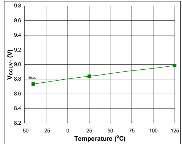
Fig. 63. V_{CC} Supply Undervoltage Positive Going Threshold vs. Temperature
