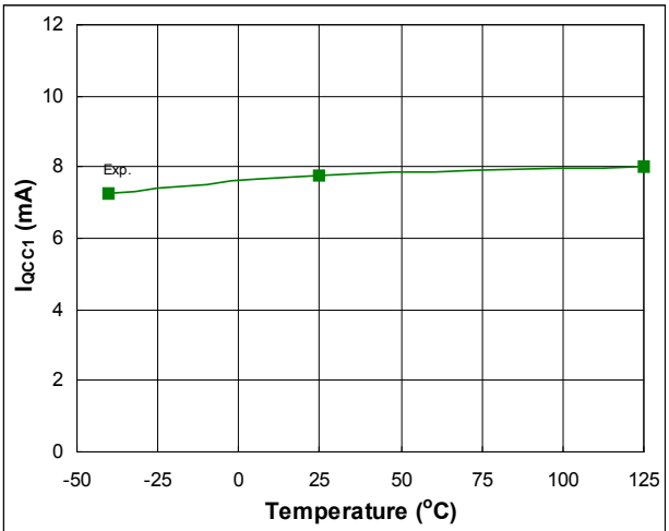
Fig. 58. Quiescent V CC Supply Current vs. Temperature
