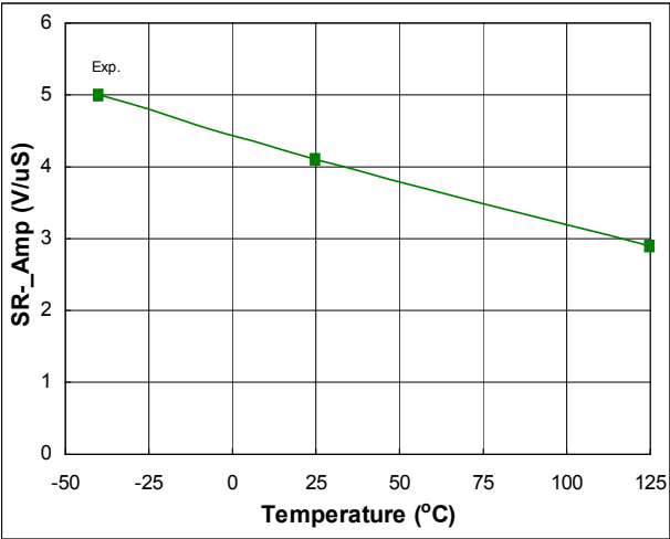
Fig. 51. Operational Amplifier Slew Rate (-) vs. Temperature
