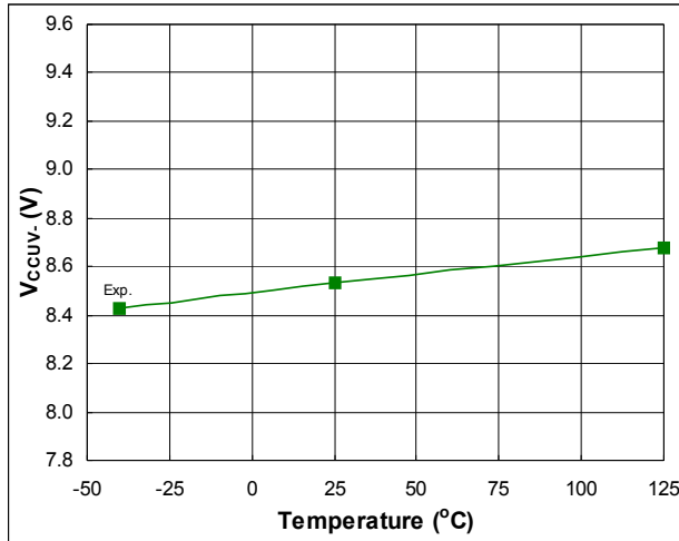
Fig. 62. V_{CC} Supply Undervoltage Negative Going Threshold vs. Temperature
