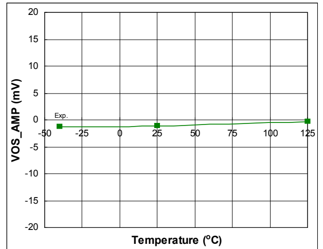
Fig. 69. Offset Opamp vs. Temperature
