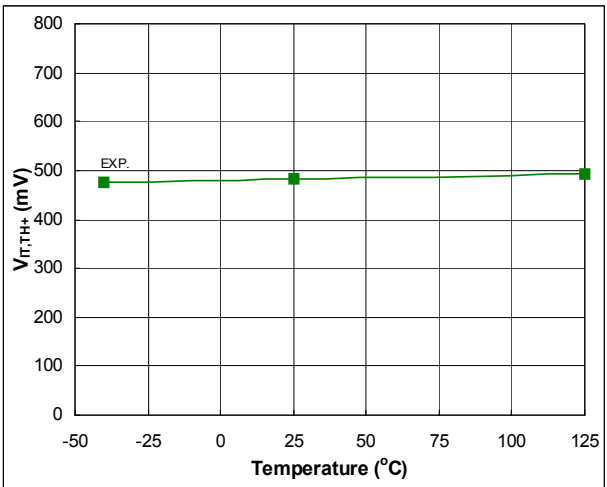
Fig. 54. ITRIP Input Positive Going Threshold vs. Temperature
