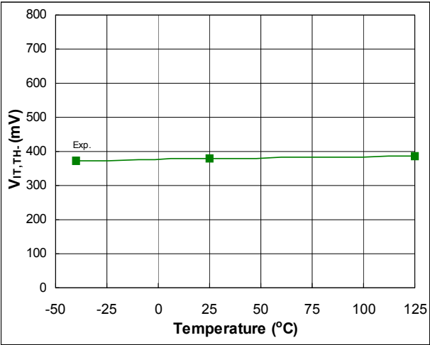
Fig. 55. ITRIP Input Negative Going Threshold vs. Temperature
