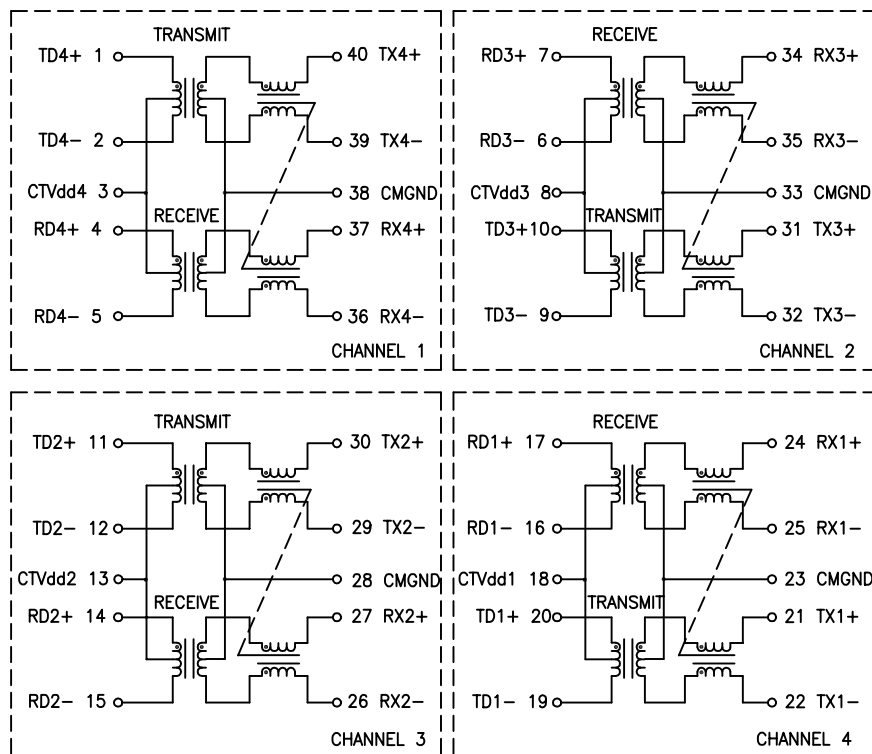
SCHEMATIC
