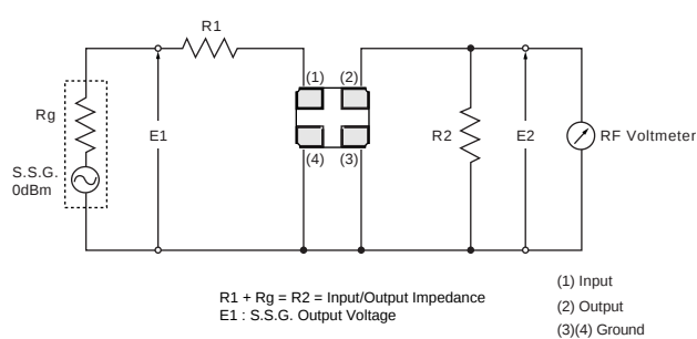
CFXCD Series
