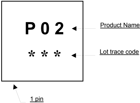
FTG (VQON16-P-0303-0.50)
