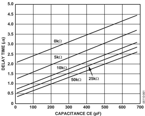
Figure 17. GPM Delay Time vs. CE Capacitance
