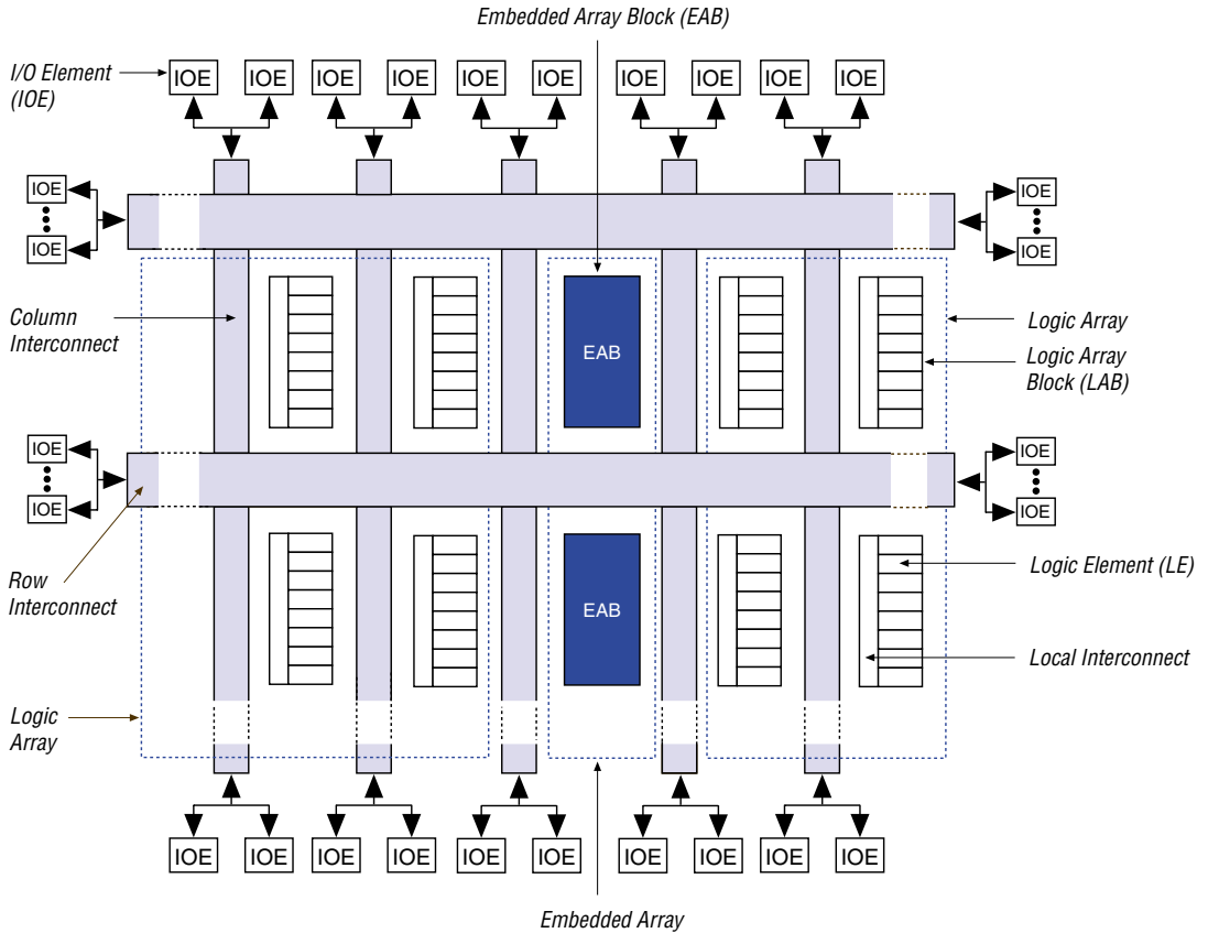
Figure 1. ACEX 1K Device Block Diagram
