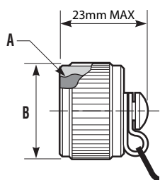
Protection cap for receptacles equipped with metallic chain, nylon cord or stainless steel rope
