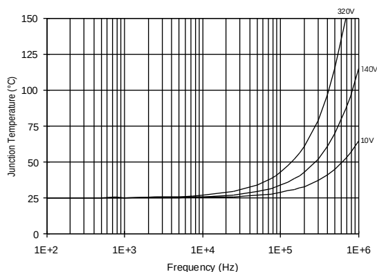
Figure 29. IR2110L6T j vs. Frequency (IRFBC30) R_{GATE} = 22\Omega , V_{CC} = 15V
