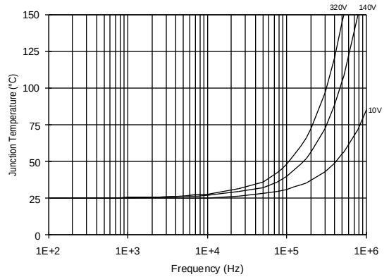
Figure 33. IR2110L6ST J vs. Frequency (IRFBC30) R GATE = 22Ω, V CC = 15V
