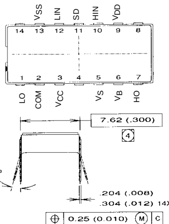
Pin Assignment
