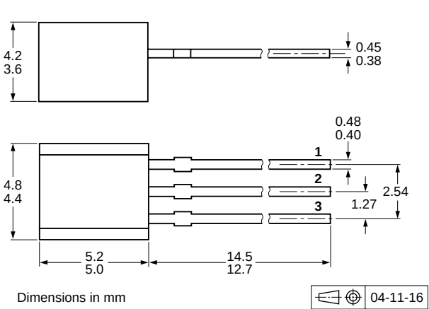
Fig 8. Package outline SOT54 (SC-43A/TO-92)
