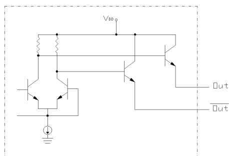
Figure 6. Standard PECL Output Configuration
