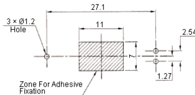
PCB / Mounting Layout
