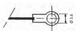
Termination of the nylon cord (or metal chain) for 00, 02 shell types protective caps.
