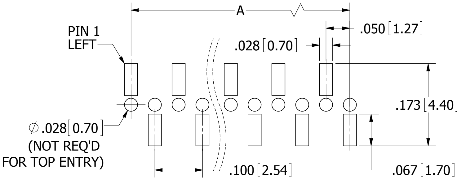
RECOMMENDED PCB LAYOUT LPPB_1NFSC-RC
