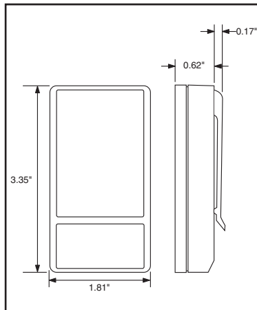
Figure 1: Package Dimensions
