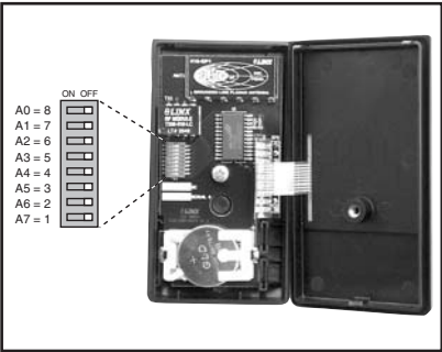
Figure 2: DIP Switch Assignments
