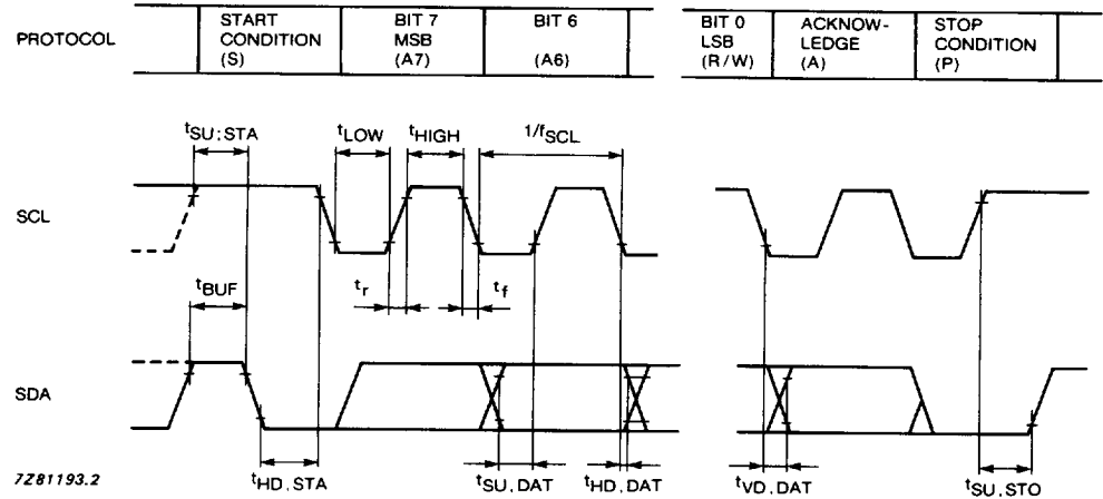
Fig.8 I 2 C-bus timing diagram.
