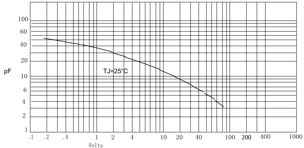
Figure 4 Junction Capacitance
