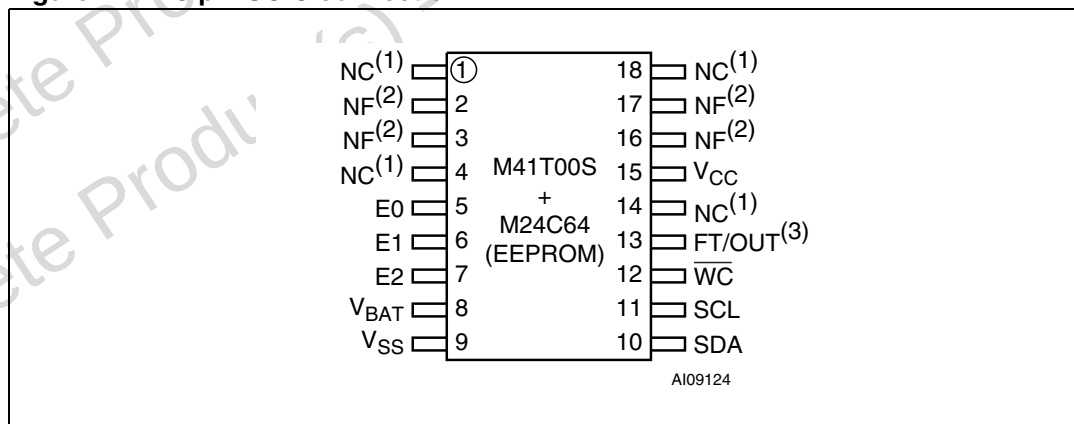
Figure 2. 18-pin SOIC connection
