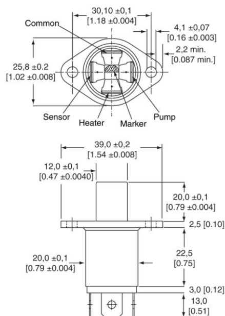
Figure 1. KGZ-10 Dimensions (For reference only: mm/in.)
