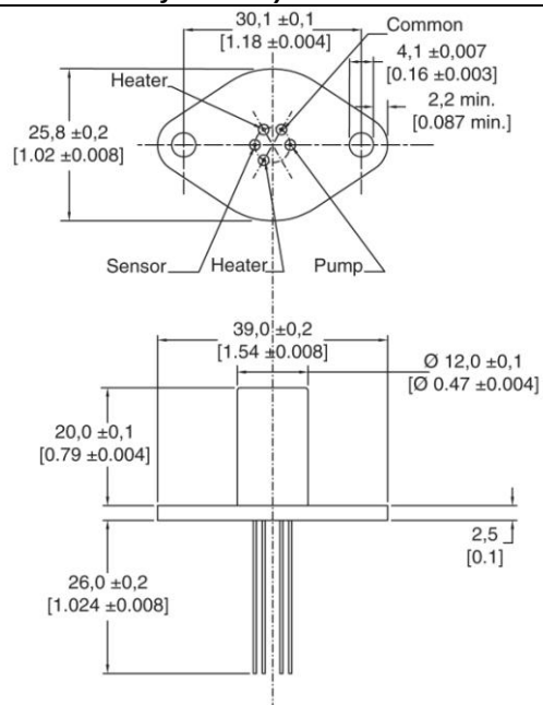
Figure 2. KGZ-10SP Dimensions (For reference only: mm/in.)
