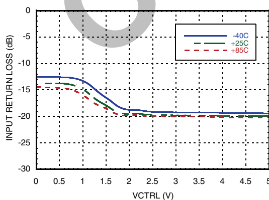
Input Return Loss vs. VCTRL [1]
