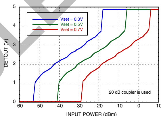
Figure 7b: DETOUT vs. input power over VSET, 2 attenuators @ 1900 MHz..
