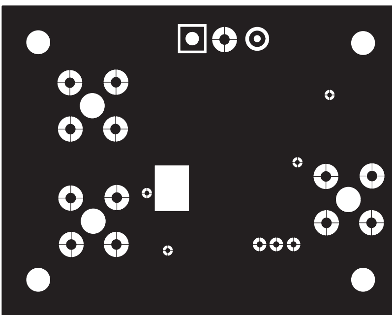
Figure 2–3. THS4081 EVM PC Board Layout: Back Side
