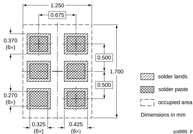
Fig 14. Reflow soldering footprint PESDxL5UF (SOT886)
