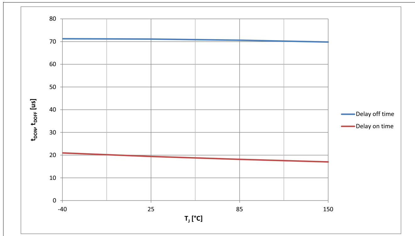
Figure 36 Typical t_{DON} , t_{DOFF} vs T_J @ V_{IN} = 5 V
