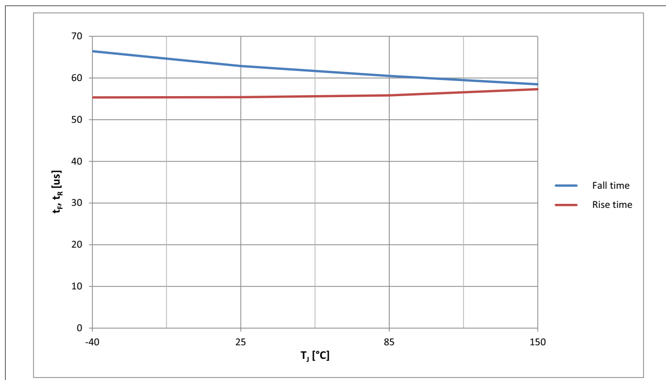
Figure 35 Typical t_F , t_R vs T_J @ V_{IN} = 5 V
