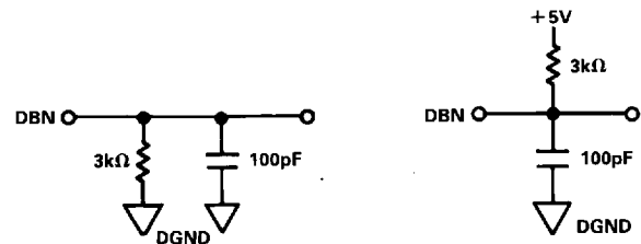
a. High-Z to V_{OH}
